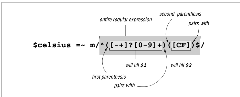
Figure 2-1: Capturing parentheses
